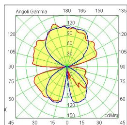
AT1P300..
